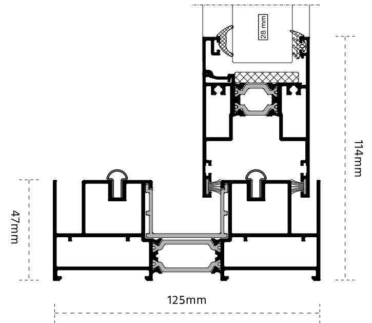
Double track (flush option)
